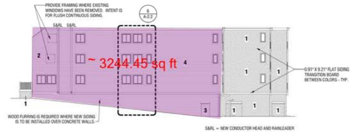
3 PARTIAL SOUTH ELEVATION
